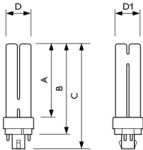
PL-C 26W/865/4P
