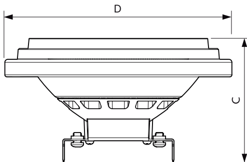
MAS LED ExpertColor 11-50W 927 AR111 40D
