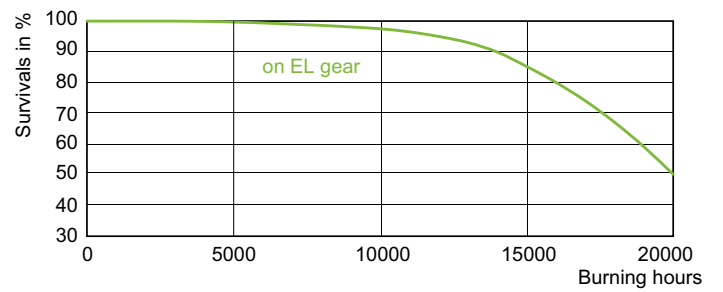
CDM-TC Elite 35W, 50W, 70W Life Expectancy /930
