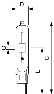
MASTERCcolour CDM-TC 35W/842 G8.5 1CT/12
