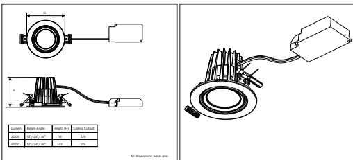
RS271B LED40/840 PSU-E WB WH
