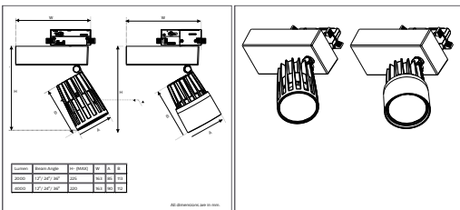
ST271T LED20/840 PSU-E NB 1C BK
