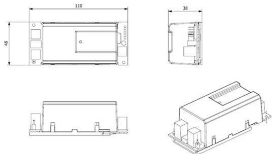
BRP710 Spare CC 4.5K Lm AIO
